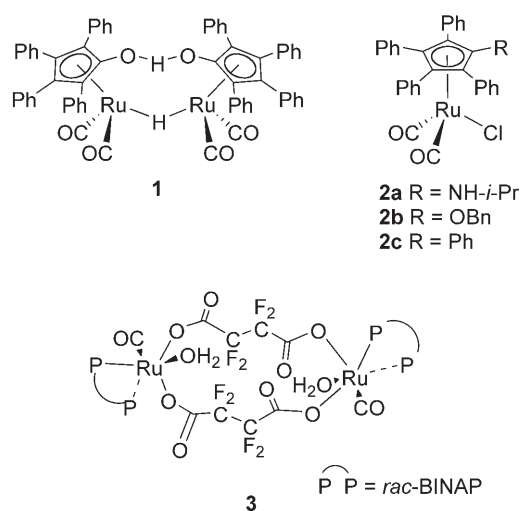
Figure 1. Ru catalysts developed for the racemization of alcohols.
