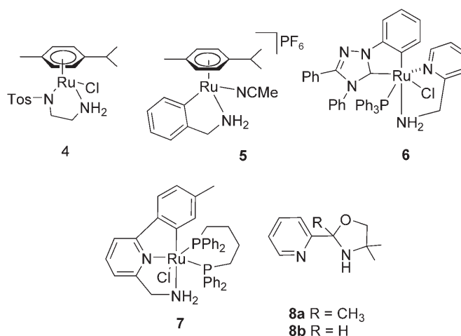
Figure 2. Ru-amino complexes and ligands used in this study.
