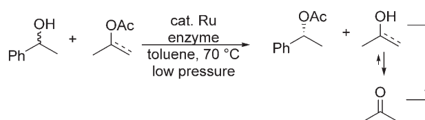
Scheme 3. Ru/enzyme combo DKR of 1-phenylethanol in the presence of isoprop(en)yl acetate.
