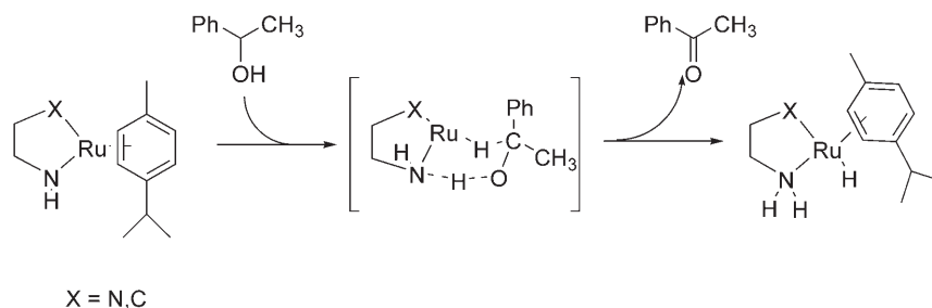
Scheme 1. Outer-sphere mechanism for hydrogen transfer catalyzed by Ru-NH ligand complexes.
