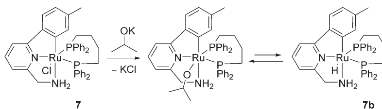
Scheme 2. Isolation of Ru-H species 7b .
